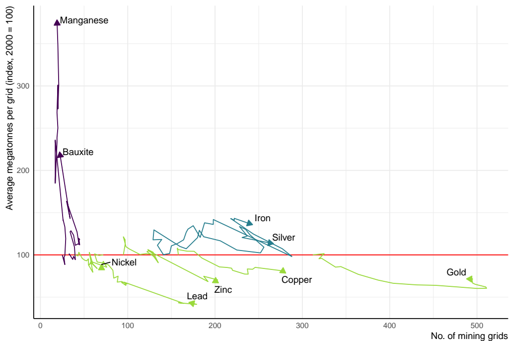
Figure A4: 2000-2019 development of the counts of 1 degree resolution mining grid cells and average extraction volumes per cell (index, 2000 = 100); starting and end points of arrows denote the years 2000 and 2019, respectively; based on SNL (2020) and UN IRP (2017) conversion factors.
