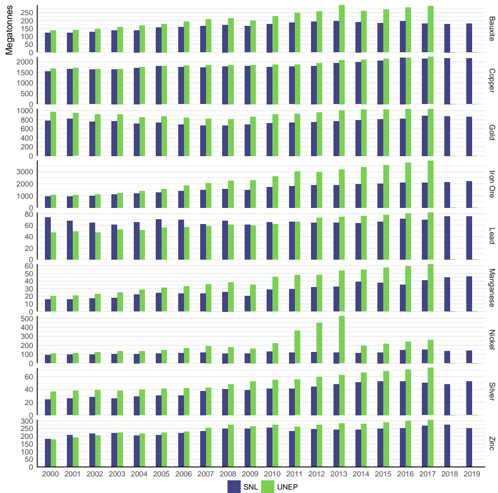
Figure A1: Globally aggregated crude ore extraction of the commodities covered in this study. Comparison of the utilised data (based on mine accounts by SNL 2020) and UNEP’s national statistics (UN IRP 2017a). UNEP 2015–2017 are projections; no data yet available for 2018 and 2019. Large deviations for nickel in 2011–2013 are driven by BGS (2021) (used as a source for UNEP’s domestic extraction statistics) reporting an extreme production increase for Indonesia over this period (followed by a rapid drop in 2014). This development is apparently not reflected in the SNL data.
