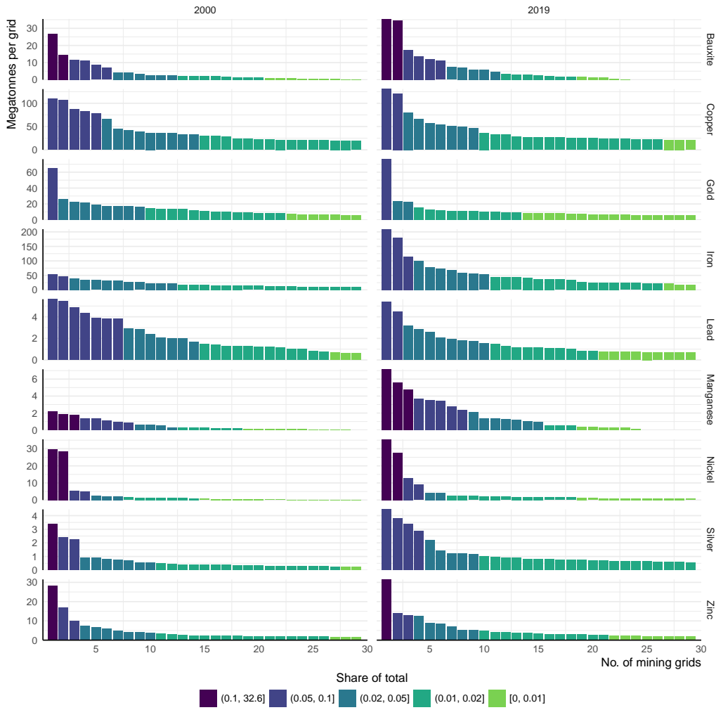
Figure A7: Metal ore extraction on a 0.25 degree resolution (i.e. about 28 \text{ km} \times 28 \text{ km} at the equator) based on SNL (2020) and UN IRP (2017) conversion factors.
