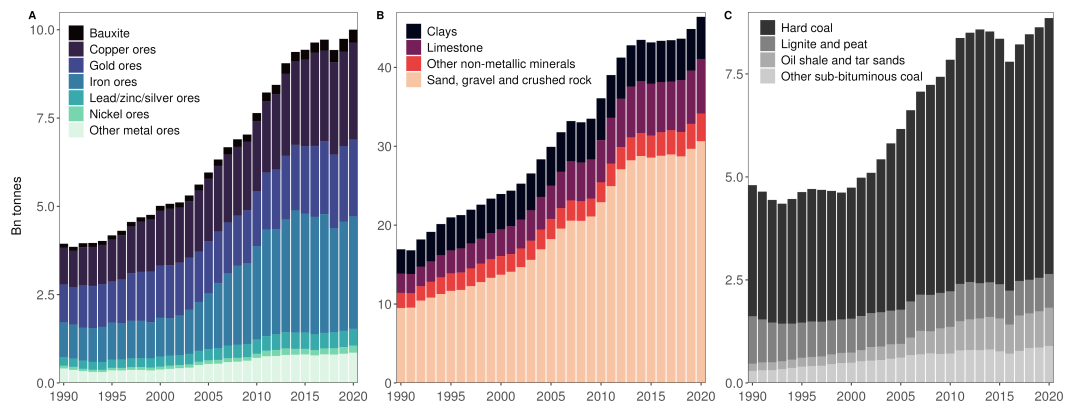
Figure 1.1: Global extraction of mined materials, 1990-2020: metallic minerals (A), non-metallic minerals (B) and mined fossil fuels (C). Data sourced from the UN IRP Material Flows Database, accessed via Release 057 of the GLORIA global environmentally-extended MRIO database (Lenzen et al. 2017; Lenzen et al. 2022).
