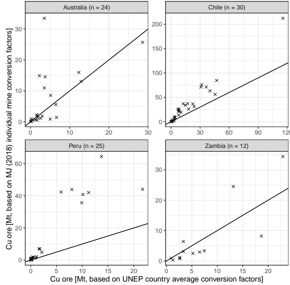
Figure A2: 2015 copper extraction estimates for each mine: UN IRP (2017) vs. Mudd and Jowitt (2018) conversion factors. Solid line indicates 45 degrees.
