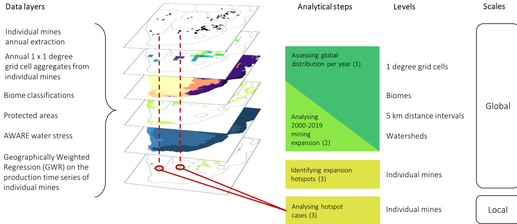
Figure 2.2: Workflow of this study, highlighting utilised spatial data, analytical steps 1-3, and respective operational level and scale of each stage. Dashed red lines represent links across layers, and solid red lines indicate syntheses of information.
